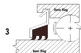
3 TRL-Seal Full cover metal shroud with triple (3) Buna-N rubber lips.
