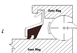
4 DBL-Seal Full cover metal shroud with double (2) Buna-N rubber lips.
