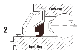
2 R-Seal Full cover metal shroud with Buna-N rubber lip plus slinger.
